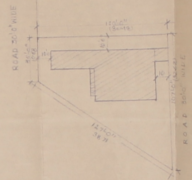
SITE PLAN SCALE 1" = 32'-0"
