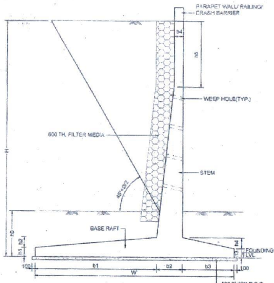
CROSS SECTION OF RETURN WALL SCALE 1:50
