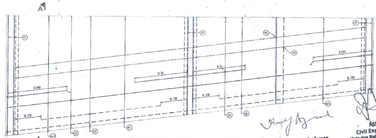
REINFORCEMENT DETAILS OF TOP SLAB SCALE - 1:50
