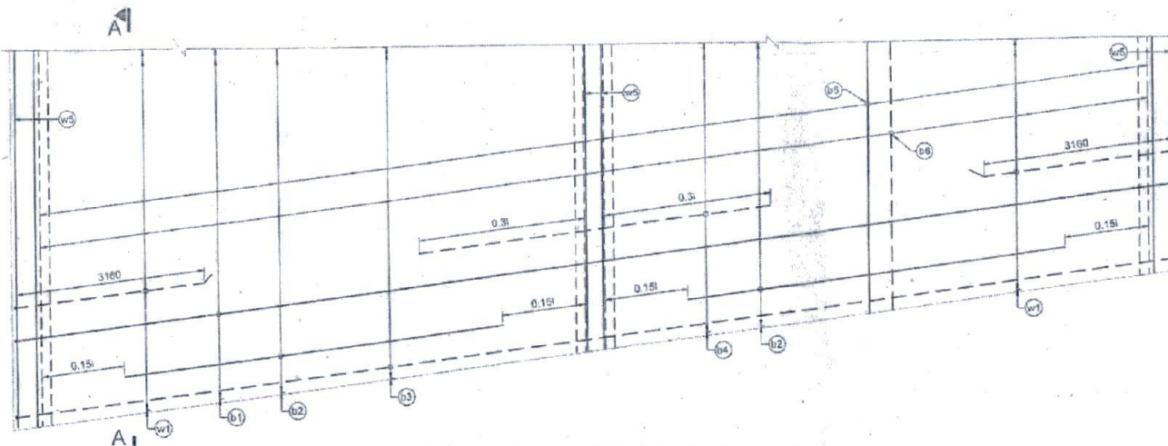
REINFORCEMENT DETAILS OF BOTTOM SLAB SCALE - 1:50
