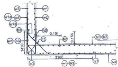
DETAIL - 3 SCALE - 1:50
