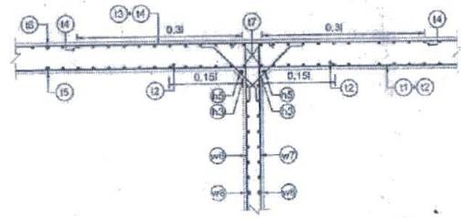
DETAIL - 2 SCALE - 1:50
