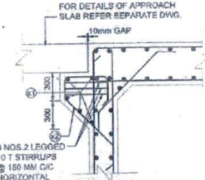
DETAIL - 5 SCALE - 1:25
