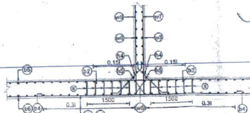
DETAIL - 4 SCALE - 1:50
