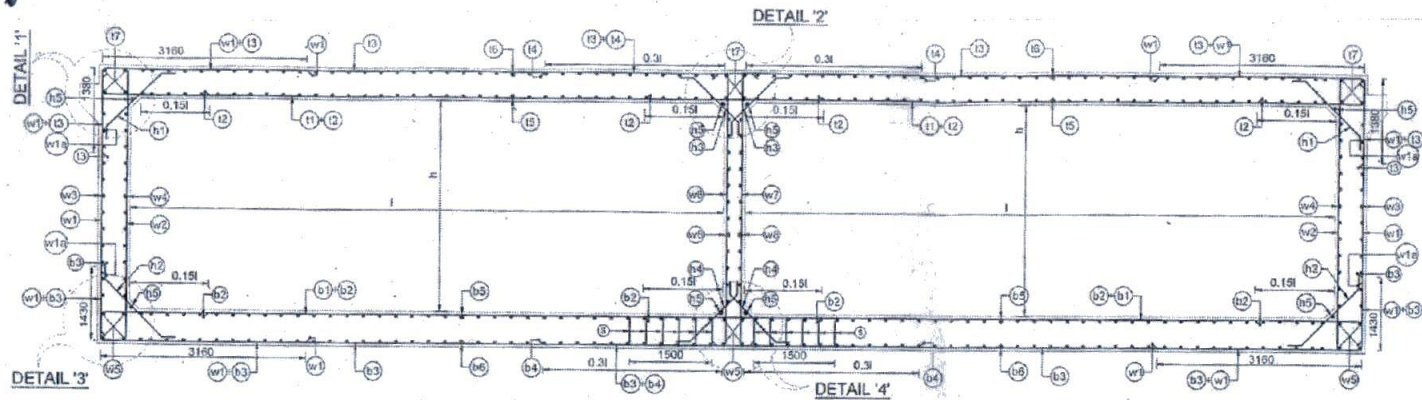
REINFORCEMENT DETAILS OF CAST IN SITU RCC BOX SCALE - 1:50
